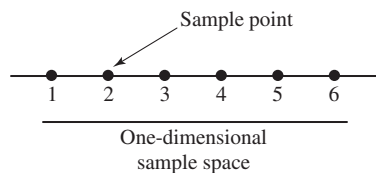
FIGURE 8.1 Sample space of the experiment of throwing a die.
