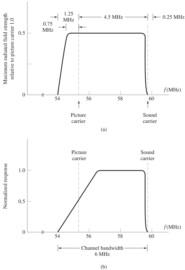
FIGURE 3.28 (a) Idealized amplitude spectrum of a transmitted TV signal. (b) Amplitude response of a VSB shaping filter in the receiver.
