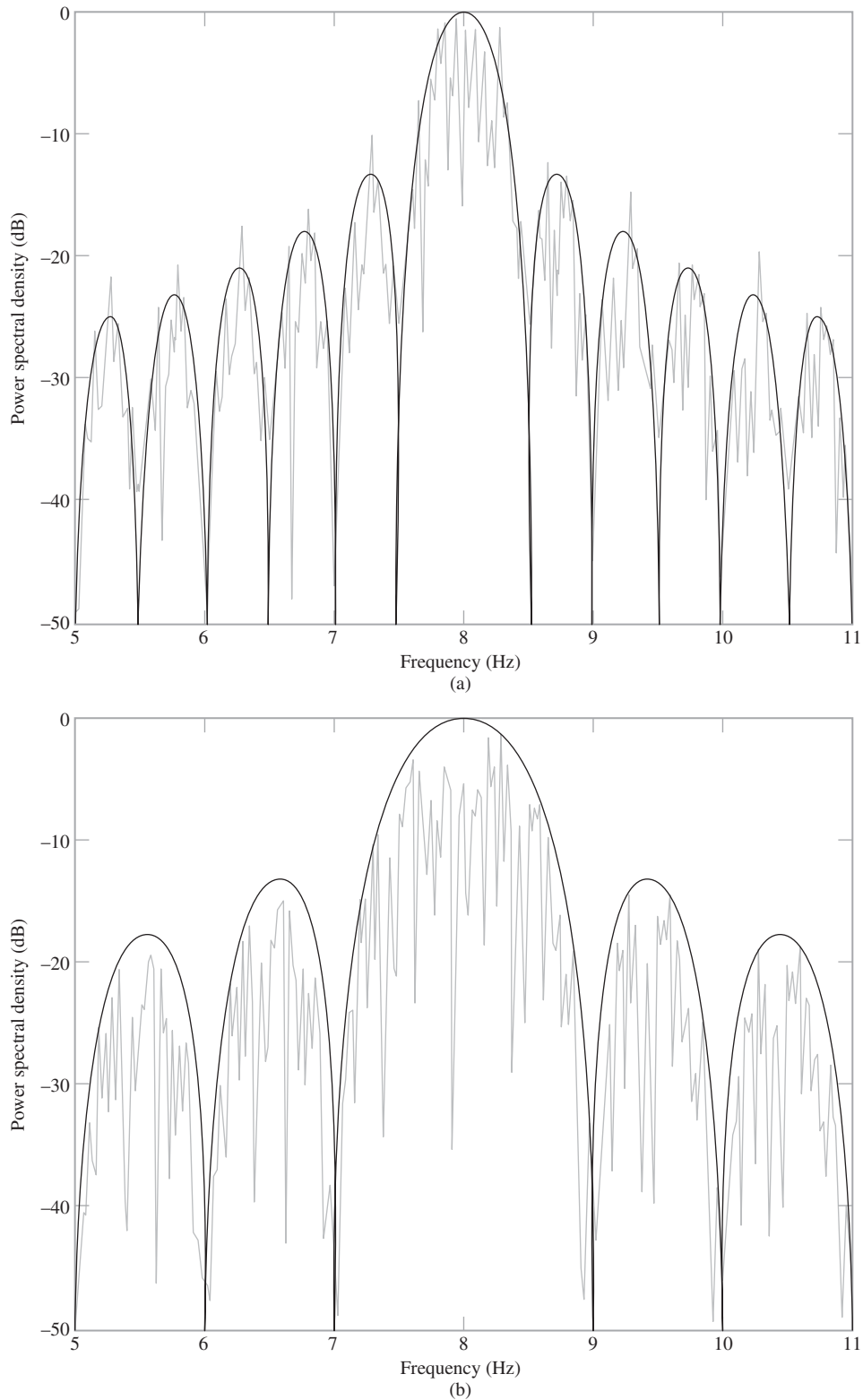
FIGURE 7.9 Power spectra of QPSK produced by square wave as the modulating signal for fixed carrier frequency and varying bit duration: (a) f_c = 8 Hz and T_b = 1 s; (b) f_c = 8 Hz and T_b = 1/2 s.
