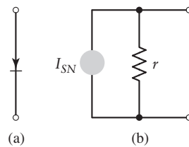
FIGURE 11.3 (a) Junction diode. (b) Shot noise model.
