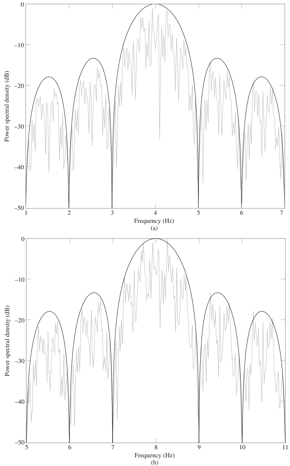
FIGURE 7.5 Power spectra of BPSK signal produced by square wave as the modulating signal for varying modulation frequency: (a) f_c = 4 Hz and T_b = 1 s; (b) f_c = 8 Hz and T_b = 1 s.
