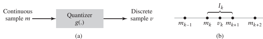
FIGURE 5.9 Description of a memoryless quantizer.
