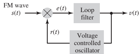
FIGURE 4.14 Block diagram of the phase-locked loop.
