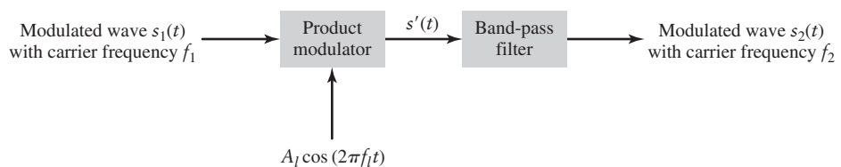
FIGURE 3.21 Block diagram of mixer.
