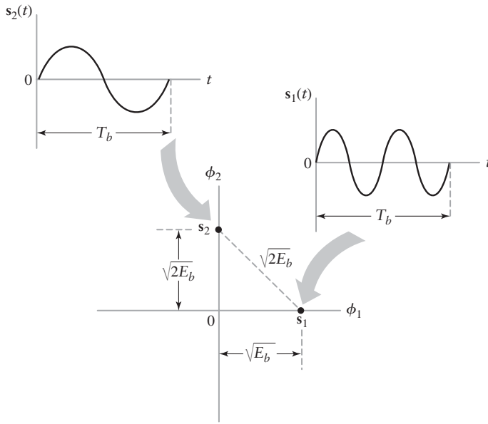
FIGURE 7.24 Mapping of BFSK onto two-dimensional signal-space diagram.
