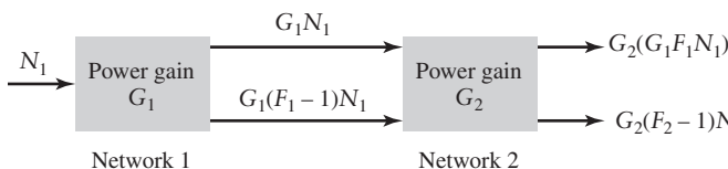
FIGURE 11.6 A cascade of two noisy networks.
