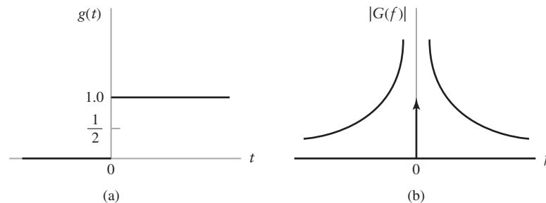
FIGURE 2.18 (a) Unit step function. (b) Amplitude spectrum.
