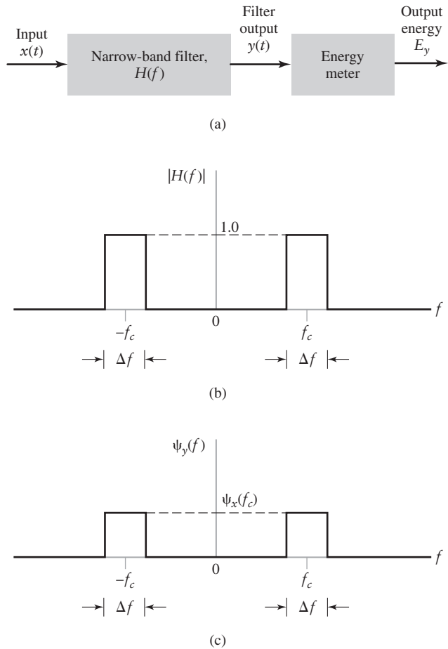
FIGURE 2.33 (a) Block diagram of system for measuring energy spectral density. (b) Idealized amplitude response of the filter. (c) Energy spectral density of the filter output.
