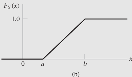
FIGURE 8.5 The uniform distribution. (a) The probability density function. (b) The distribution function.
