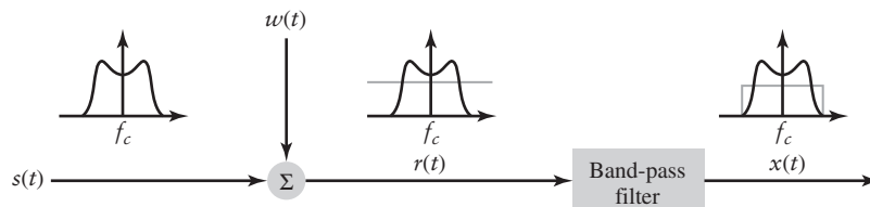
FIGURE 9.1 Block diagram of signal plus noise before and after filtering, showing spectra at each point.
