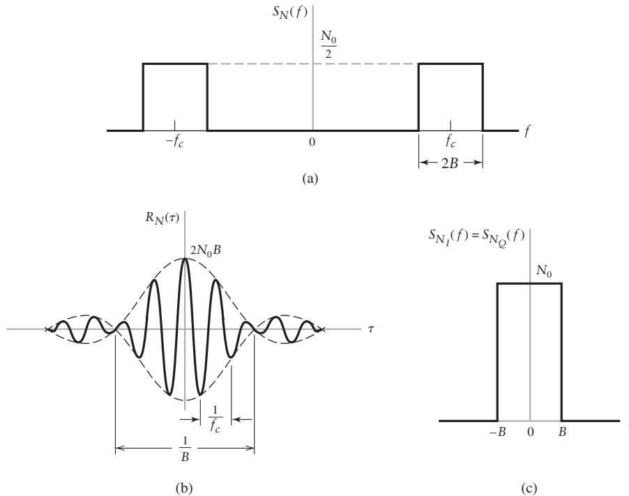
FIGURE 8.23 Characteristics of ideal band-pass filtered white noise. (a) Power spectral density. (b) Autocorrelation function. (c) Power spectral density of in-phase and quadrature components.
