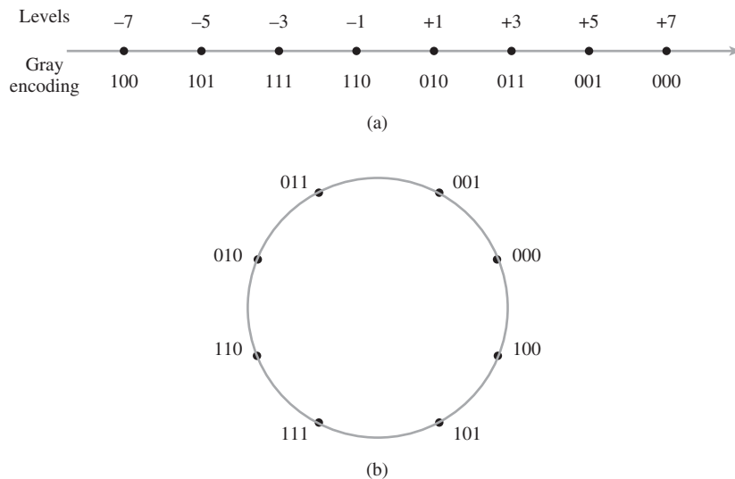
FIGURE 10.15 Gray-encoding of (a) 8-ary PAM and (b) 8-PSK.
